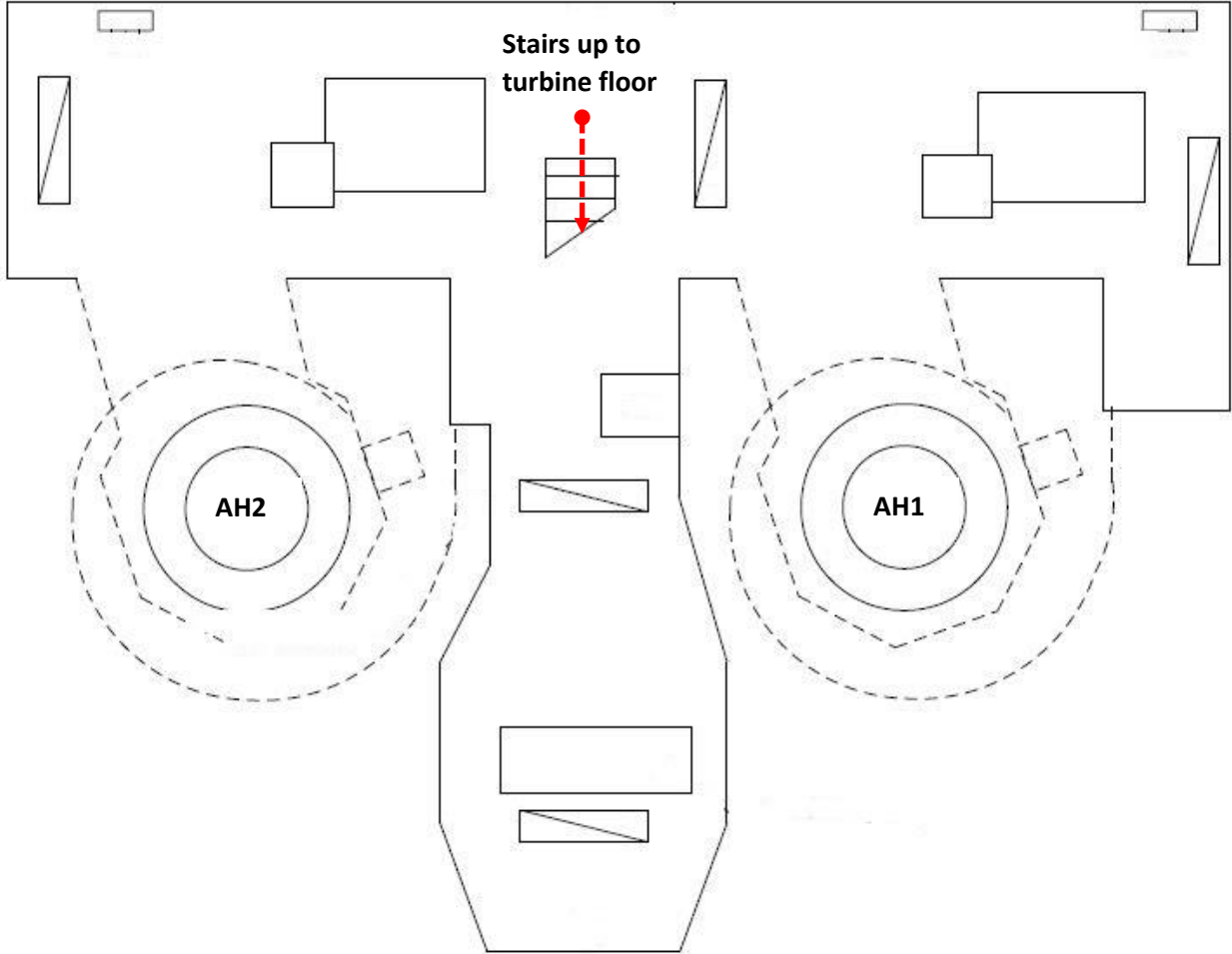
AISHIHIK HYDRO POWERHOUSE EMERGENCY EXIT ROUTE – TIV FLOOR
