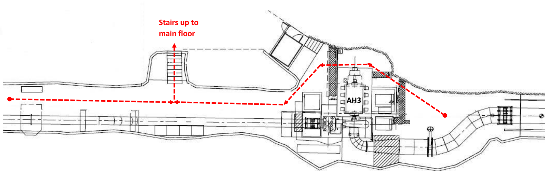
AISHIHK HYDRO POWERHOUSE EMERGENCY EXIT ROUTE – AH3 TURBINE FLOOR
