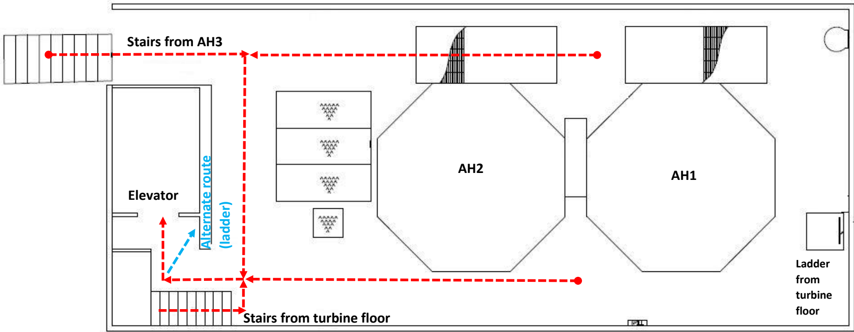
AISHIHIK HYDRO POWERHOUSE EMERGENCY EXIT ROUTES – MAIN FLOOR
