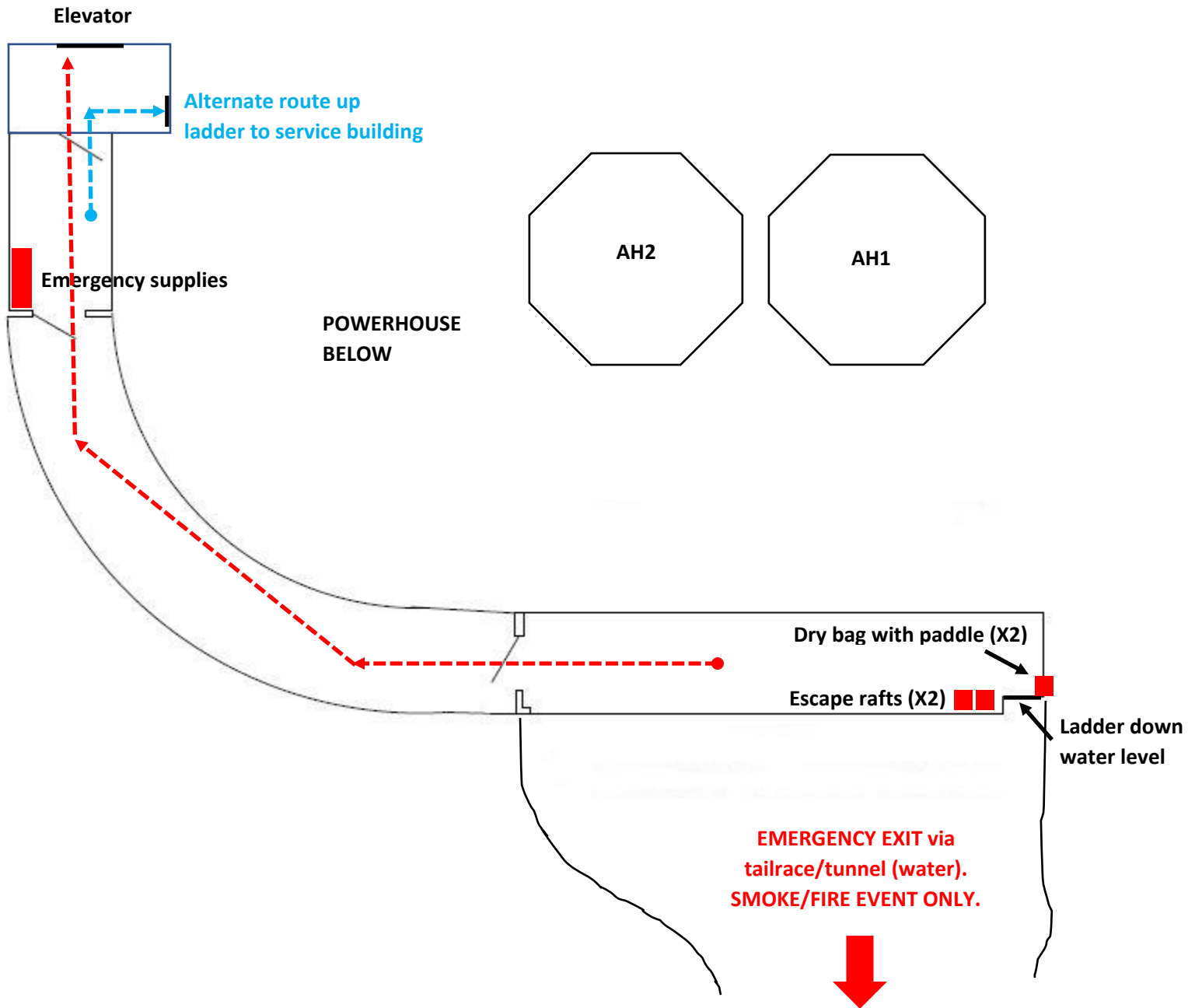
AISHIHIK HYDRO POWERHOUSE EMERGENCY EXIT ROUTE – SURGE CHAMBER
