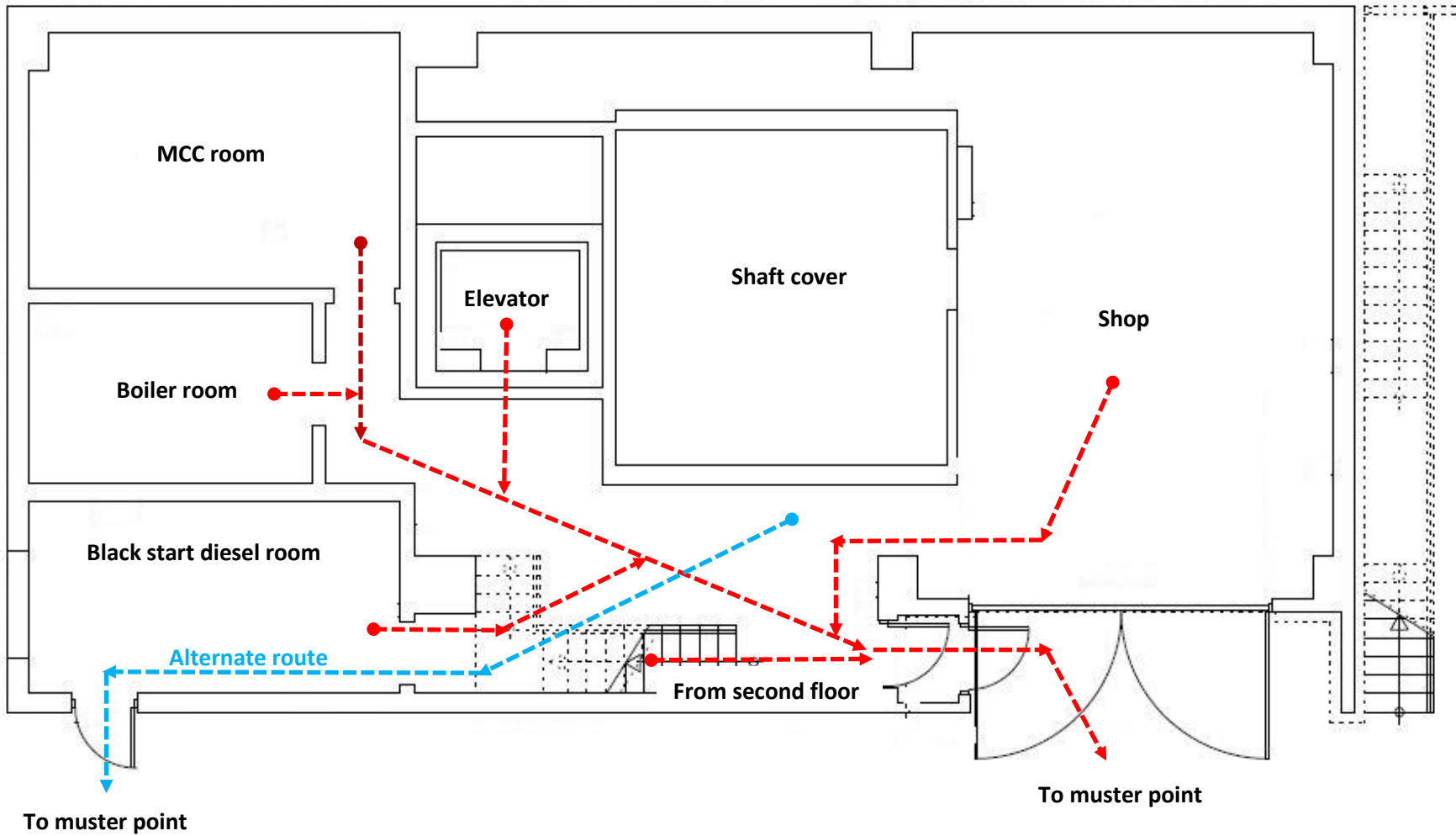
AISHIHIK HYDRO SERVICE BUILDING EMERGENCY EXIT ROUTES – MAIN FLOOR
